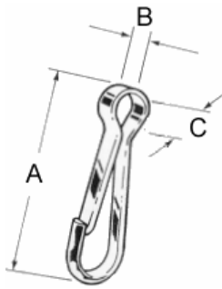
Snap Hook
