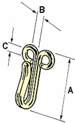
Wire Hook With Slot
