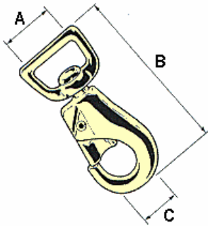
Snap Hook AK5
